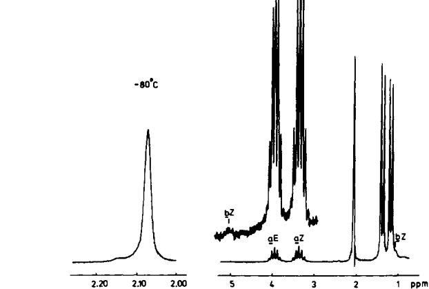
Figure 3. NMR spectra of 3 in dichlorofluoromethane.
