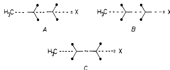
Scheme V
