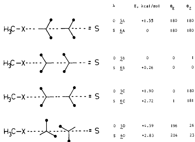
Figure 5. Calculated minimum energy conformations and conformational energies of 5 and 6 .
